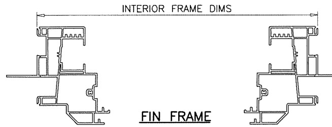
FLUSH FRAME
