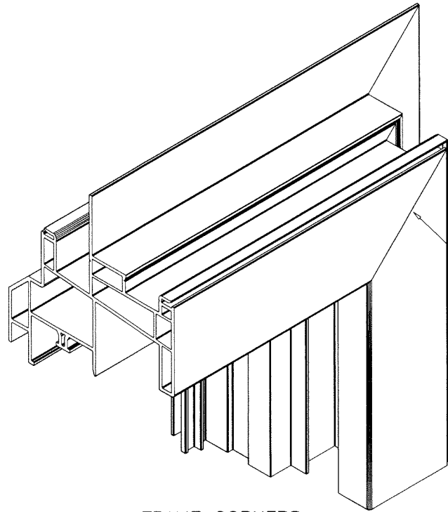
FRAME CORNERS
